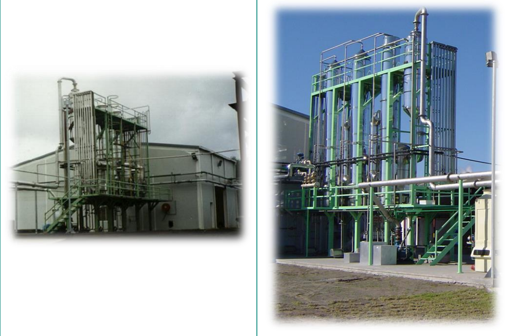
Triple Effect Long Tube Falling Film Evaporator For Pineapple located at Collondale Cannery Co., Ltd. South Africa
