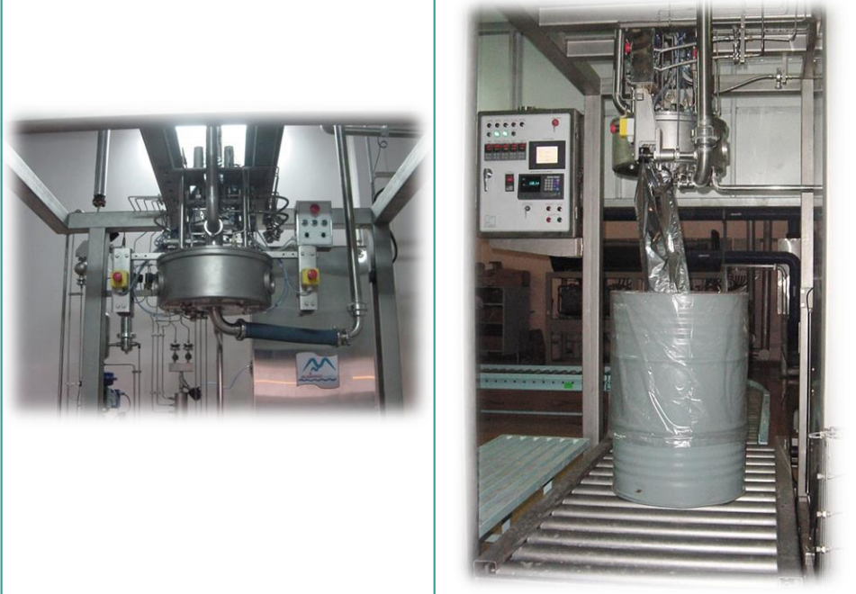
Aseptic Bulk Filler – Single Head located at Central Interfood Co., Ltd. Kanchanaburi, Thailand
